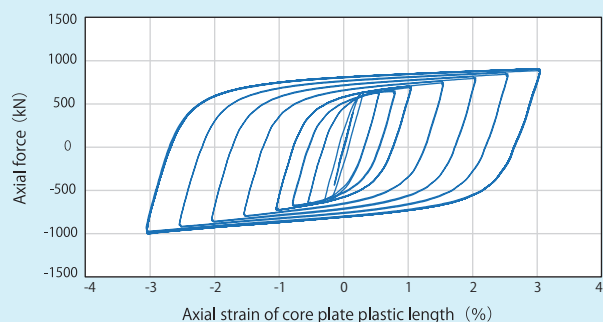
Hysteresis curve (− : compression, + : tension)
